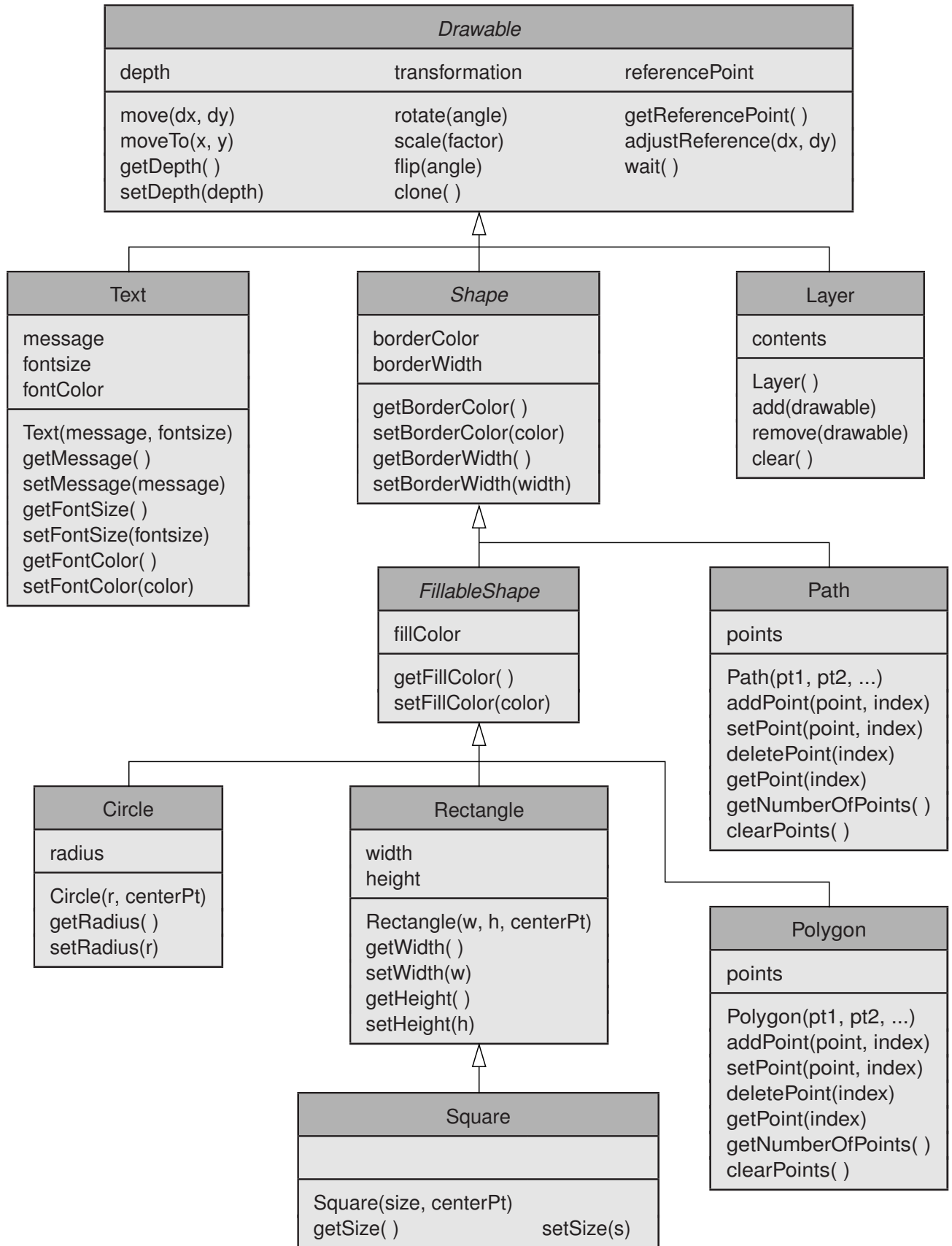
FIGURE 3.4: An overview of the Drawable objects.
